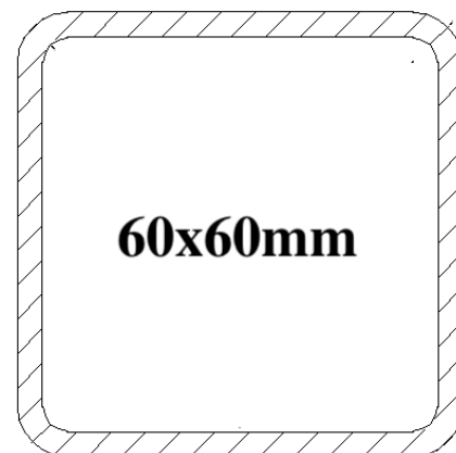
POST SECTION
